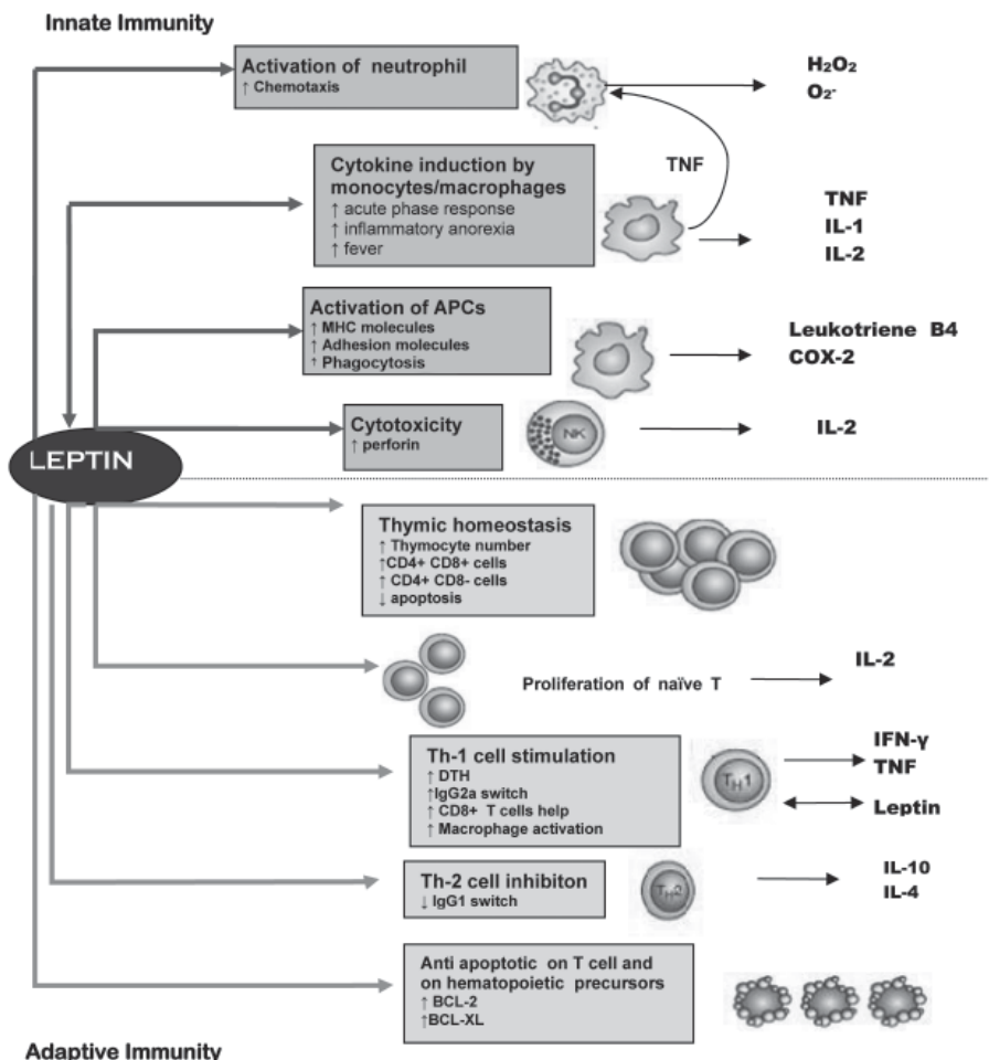
Figure 4 Effects of leptin on innate and adaptive immune responses. In innate immunity, leptin modulates the activity and function of neutrophils by increasing chemotaxis and the secretion of oxygen radicals through direct and indirect mechanisms. Leptin increases phagocytosis by monocytes/macrophages and enhances the secretion of pro-inflammatory mediators of the acute-phase response and the expression of adhesion molecules. On natural killer (NK) cells, leptin increases cytotoxic ability and the secretion of perforin and interleukin-2 (IL-2). In adaptive immunity, leptin affects the generation, maturation, and survival of thymic T cells by reducing their rate of apoptosis. On naive T-cell responses, leptin increases proliferation and IL-2 secretion. On memory T cells, leptin promotes the switch towards T helper (Th)1-cell immune responses by increasing interferon- \gamma (IFN- \gamma ) and TNF secretion. This process is then sustained by an autocrine loop of leptin secretion by Th1 cells. Leptin has anti-apoptotic effects on mature T cells and on haematopoietic precursors (adapted from La Cava et al., 2004). 55
