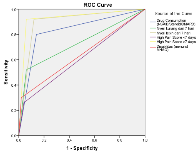
Picture 1. ROC Curve of COPCORD Questionnaire Points against Rheumatic Disease Diagnosis
